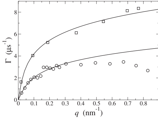
FIG. 1. Dispersion relations for the slower relaxation mode of stacks of DMPC lipid membranes at 30 °C (circles) and 19 °C (squares). (Data taken from Ref. [10].) The solid lines are fits to Eq. (2) with d=5.4 nm, \eta_M=0.016 Pa s, \Theta=110 , and \gamma=5.4 mN/m (lower curve); d=5.6 nm, \eta_M=0.016 Pa s, \Theta=350 , and \gamma=28 mN/m (upper curve). The values of d and \eta_M are taken from Ref. [10]; \Theta and \gamma are fitting parameters.
